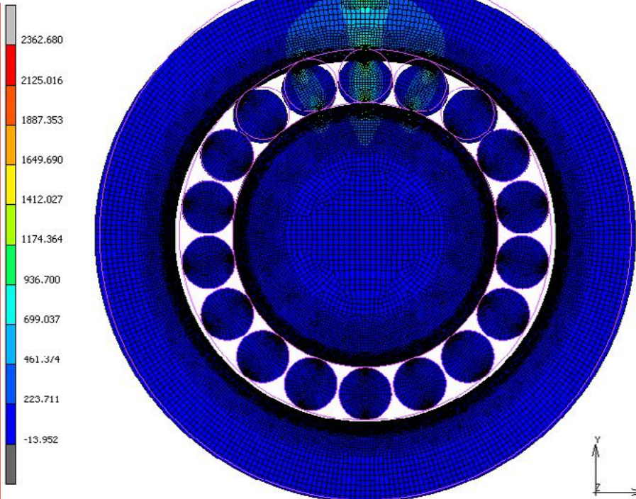
Icase3_1 Equivalent Von Mises Stress
